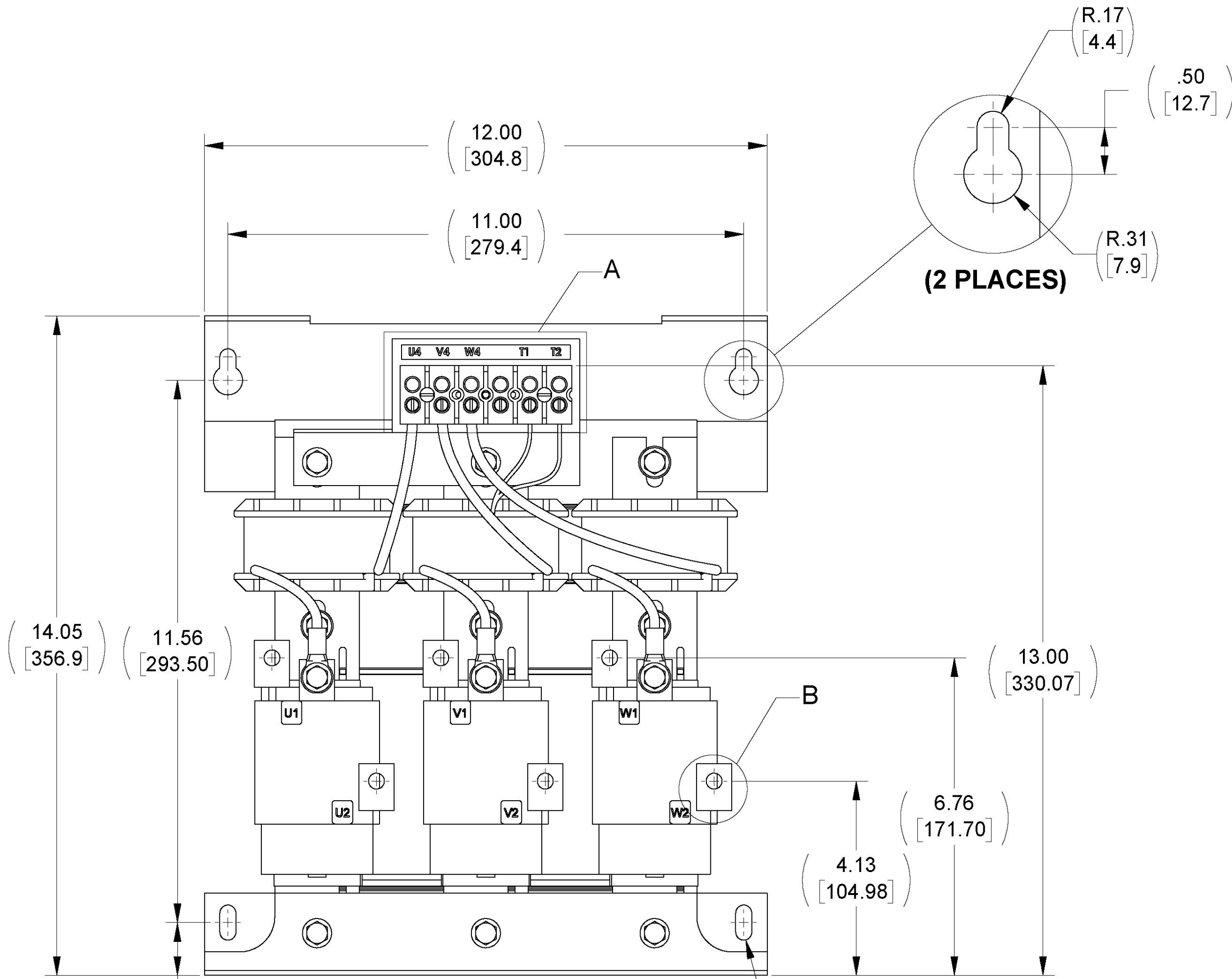
FRONT VIEW
