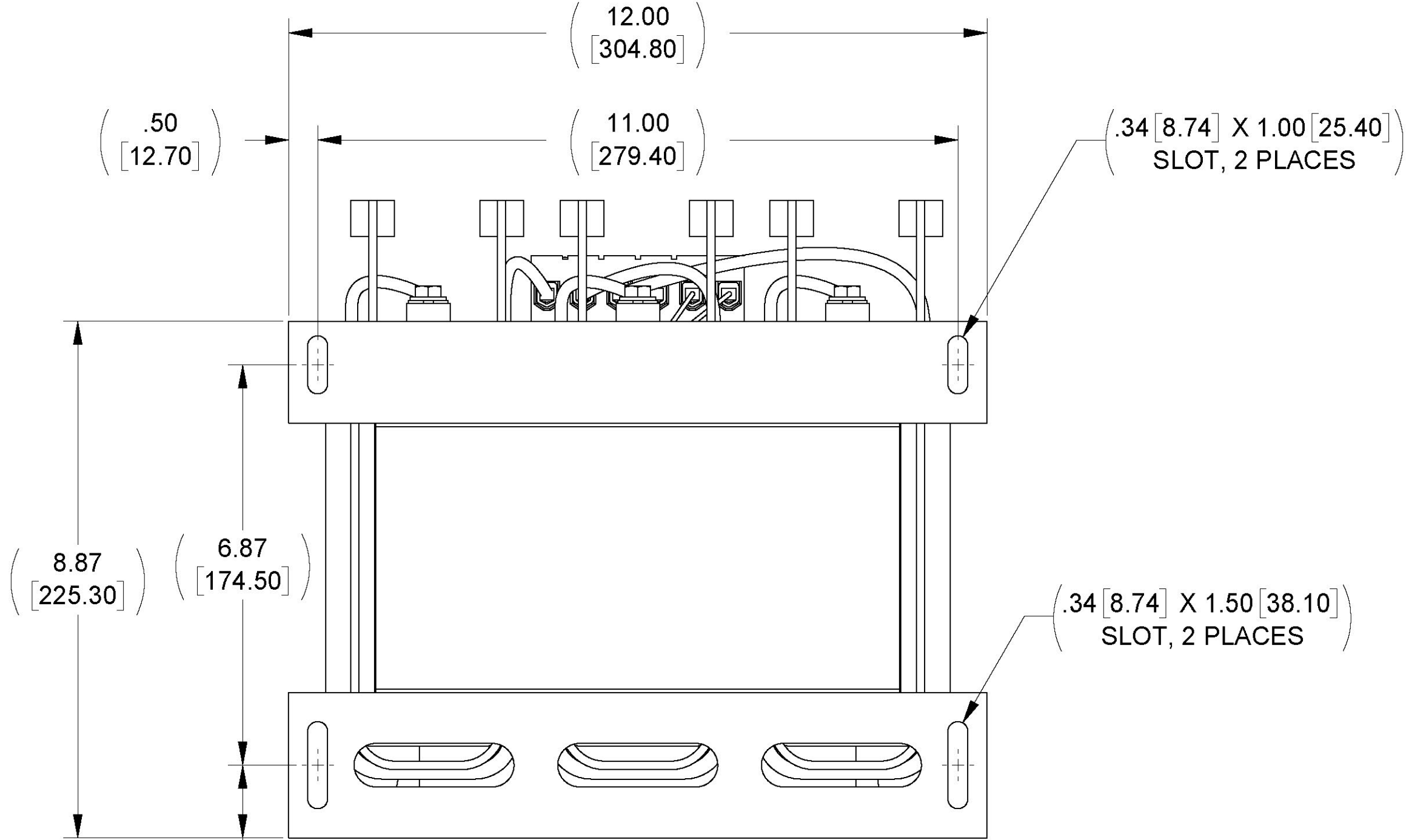
BOTTOM VIEW
