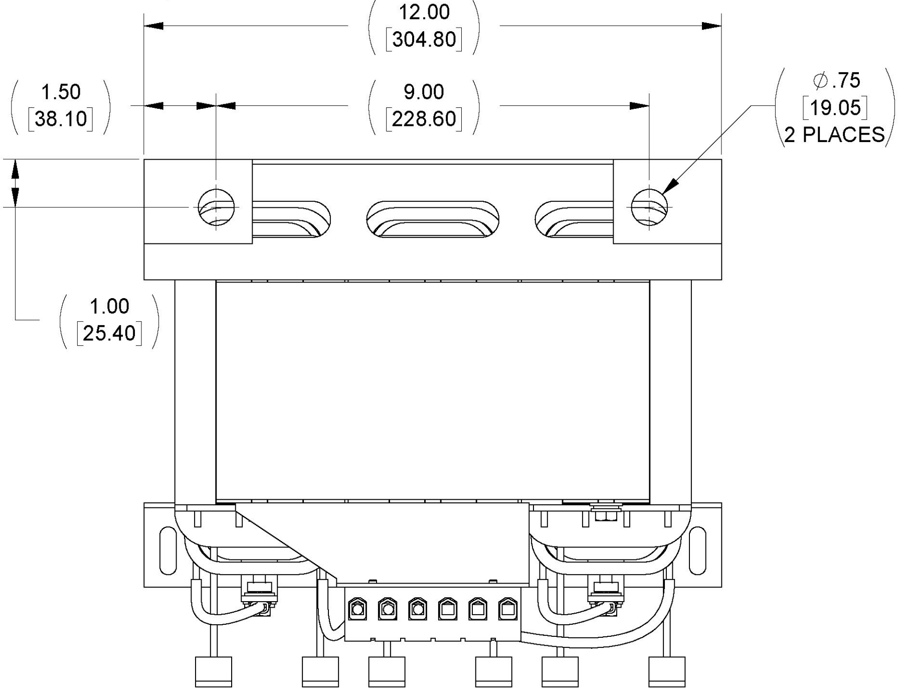
TOP VIEW
