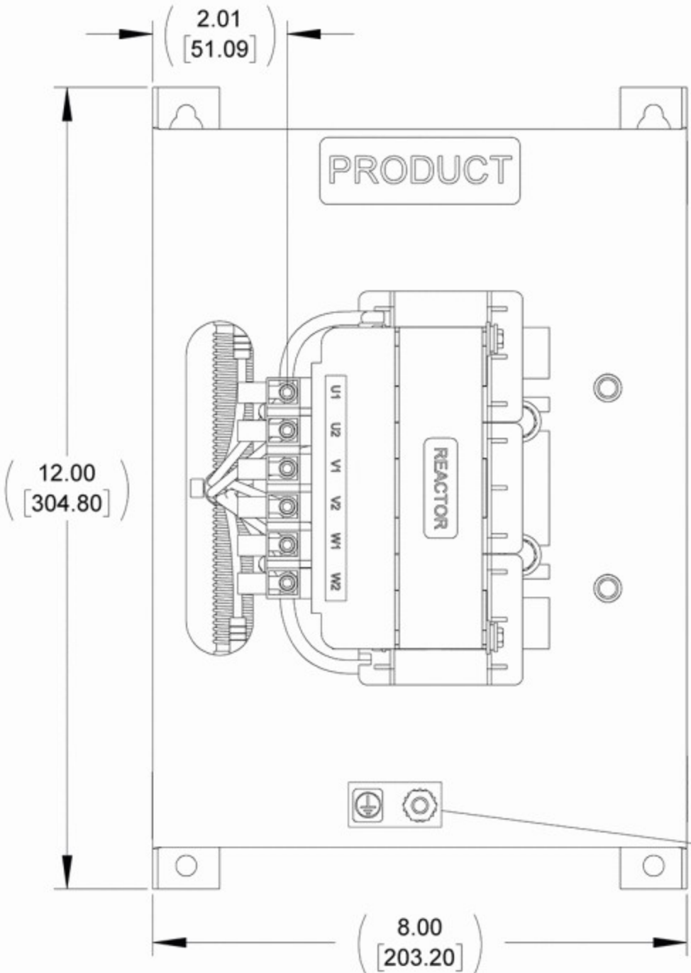
FRONT VIEW
