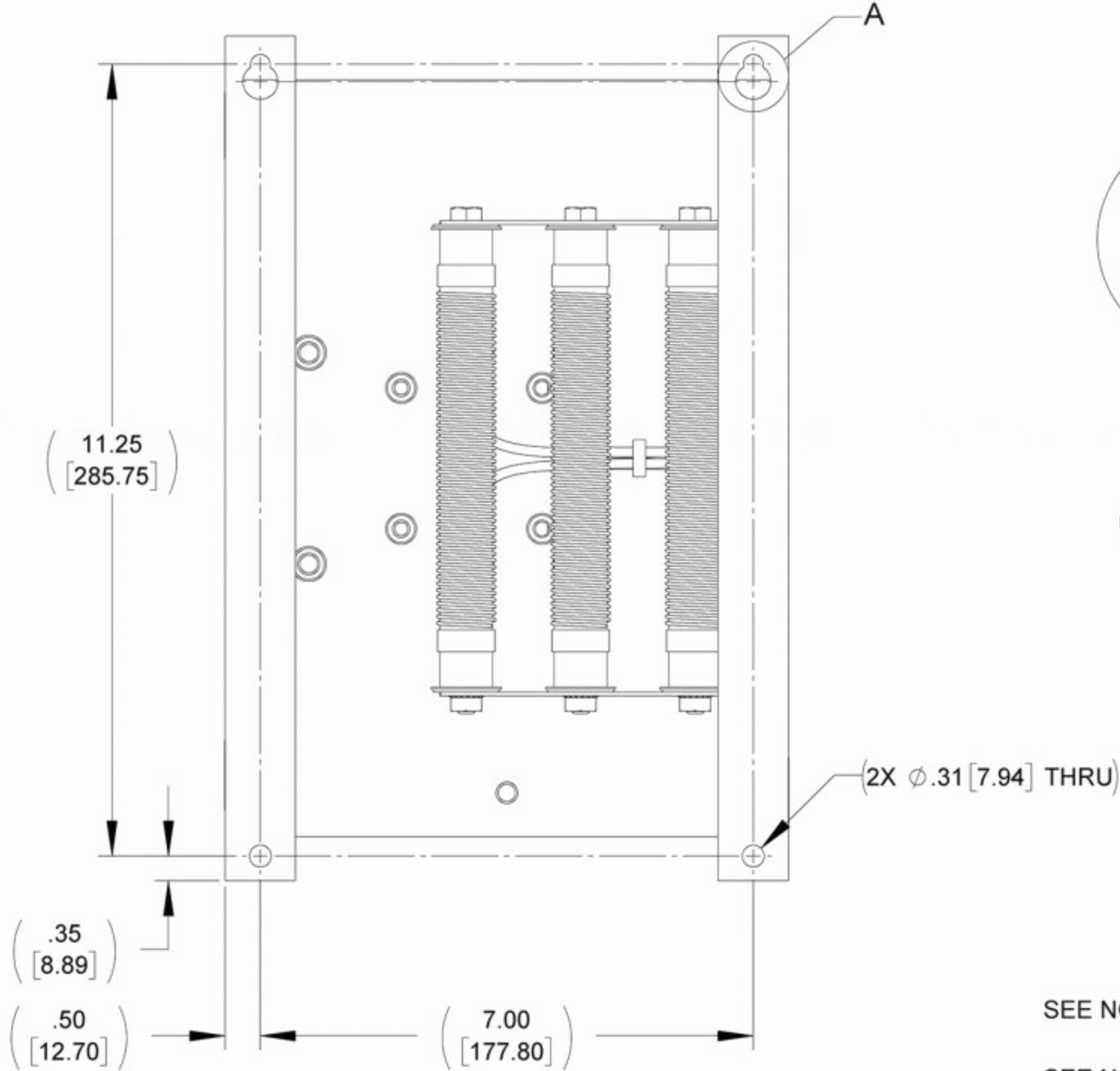
BACK VIEW
