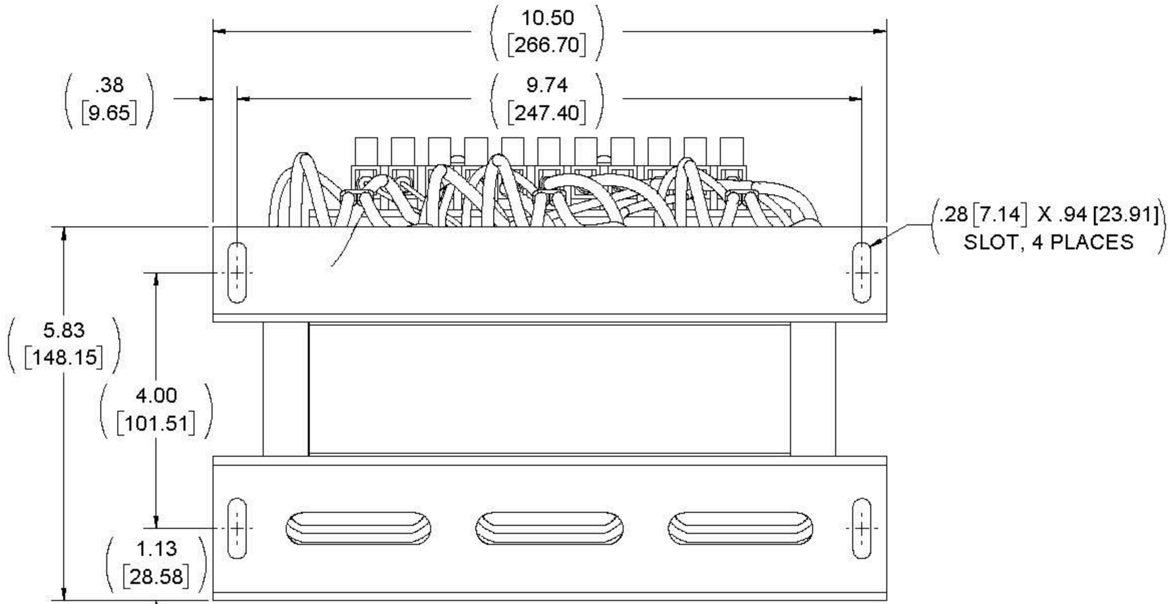
BOTTOM VIEW
