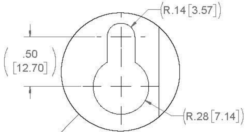
DETAIL A (2 PLACES)
