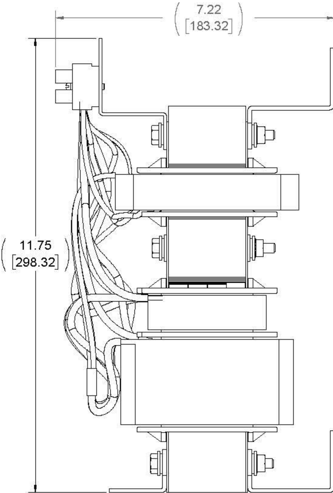
RIGHT SIDE VIEW
