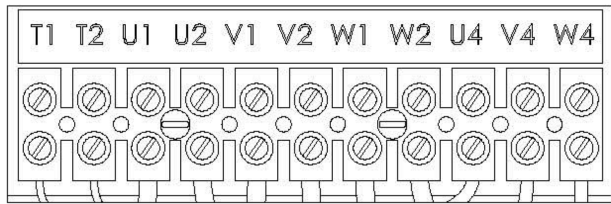
CUSTOMER CONNECTION DETAIL VIEW
