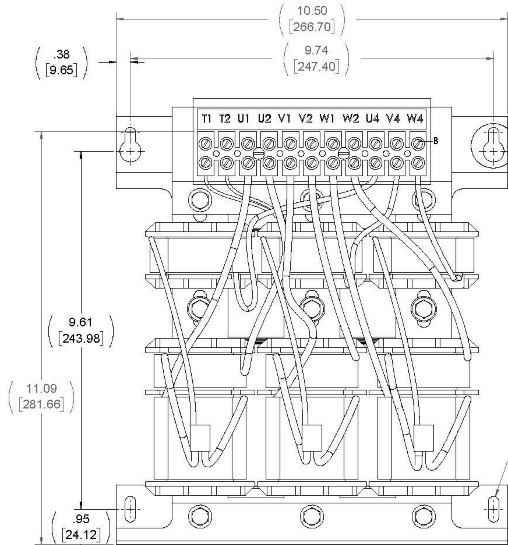
FRONT VIEW
