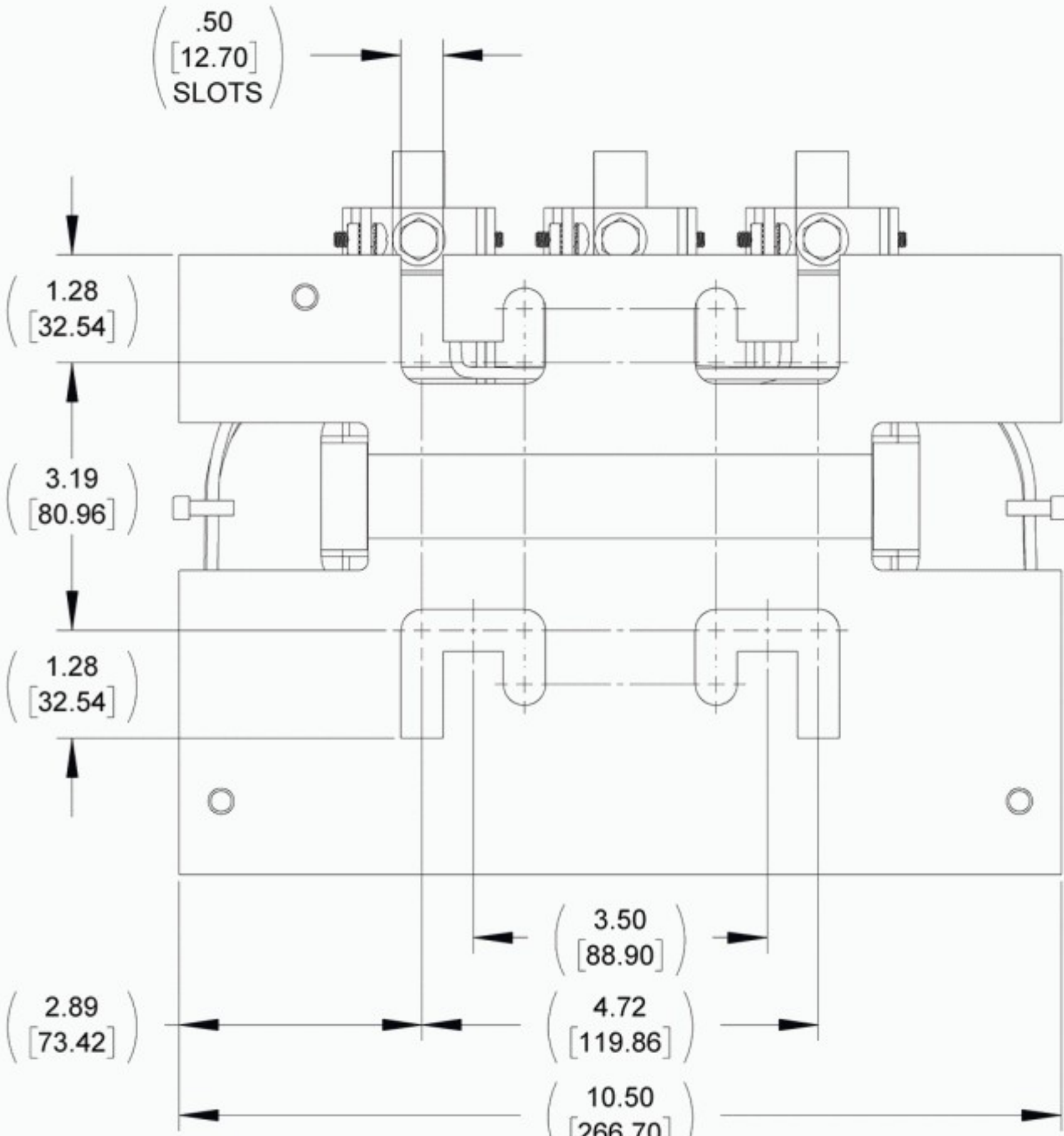
BOTTOM VIEW
