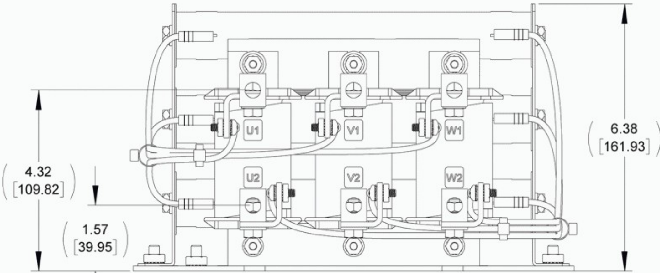
FRONT VIEW
