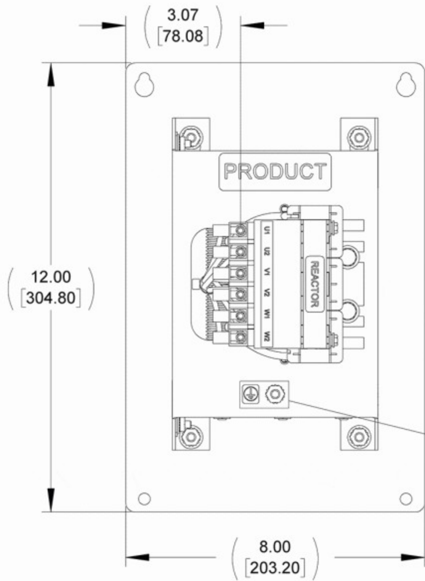
FRONT VIEW
