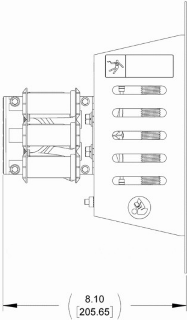
SIDE VIEW
