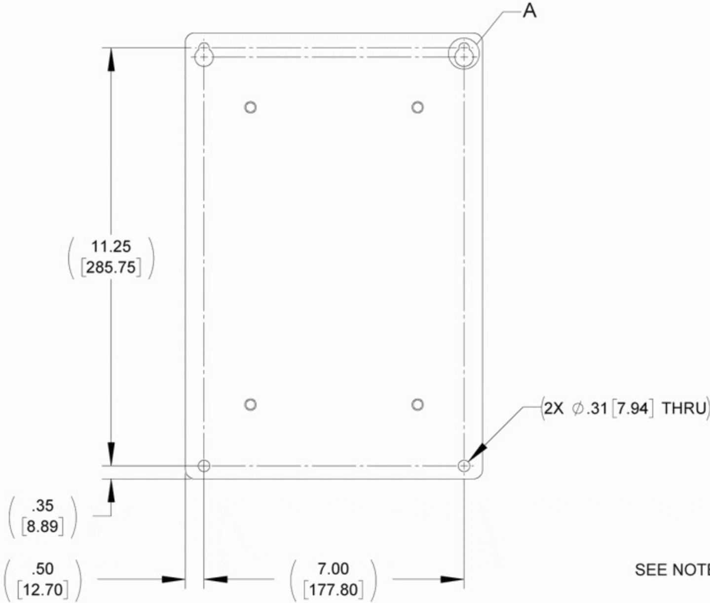
BACK VIEW
