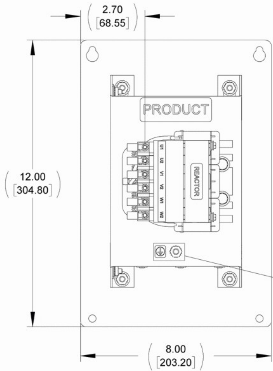
FRONT VIEW
