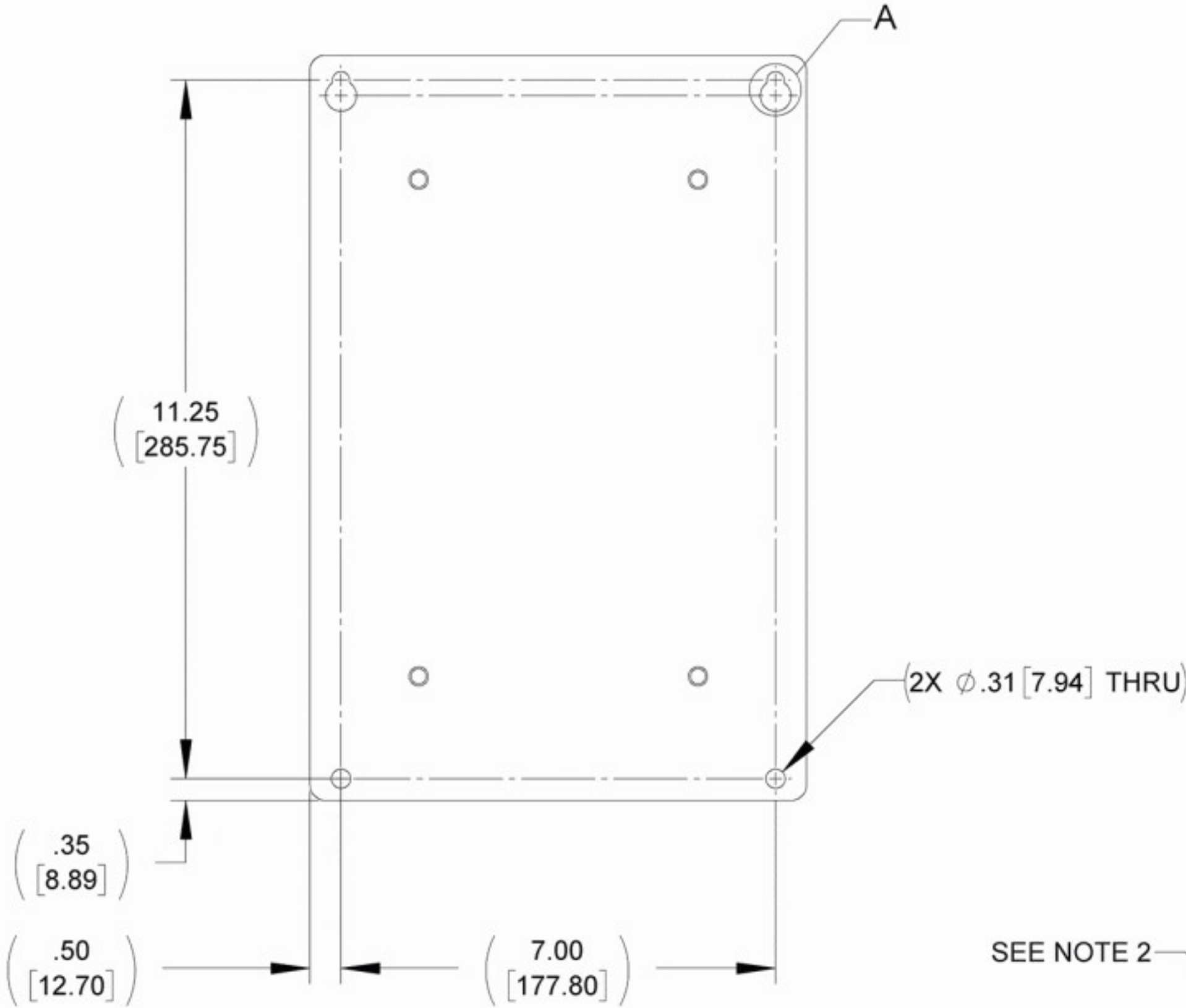
BACK VIEW
