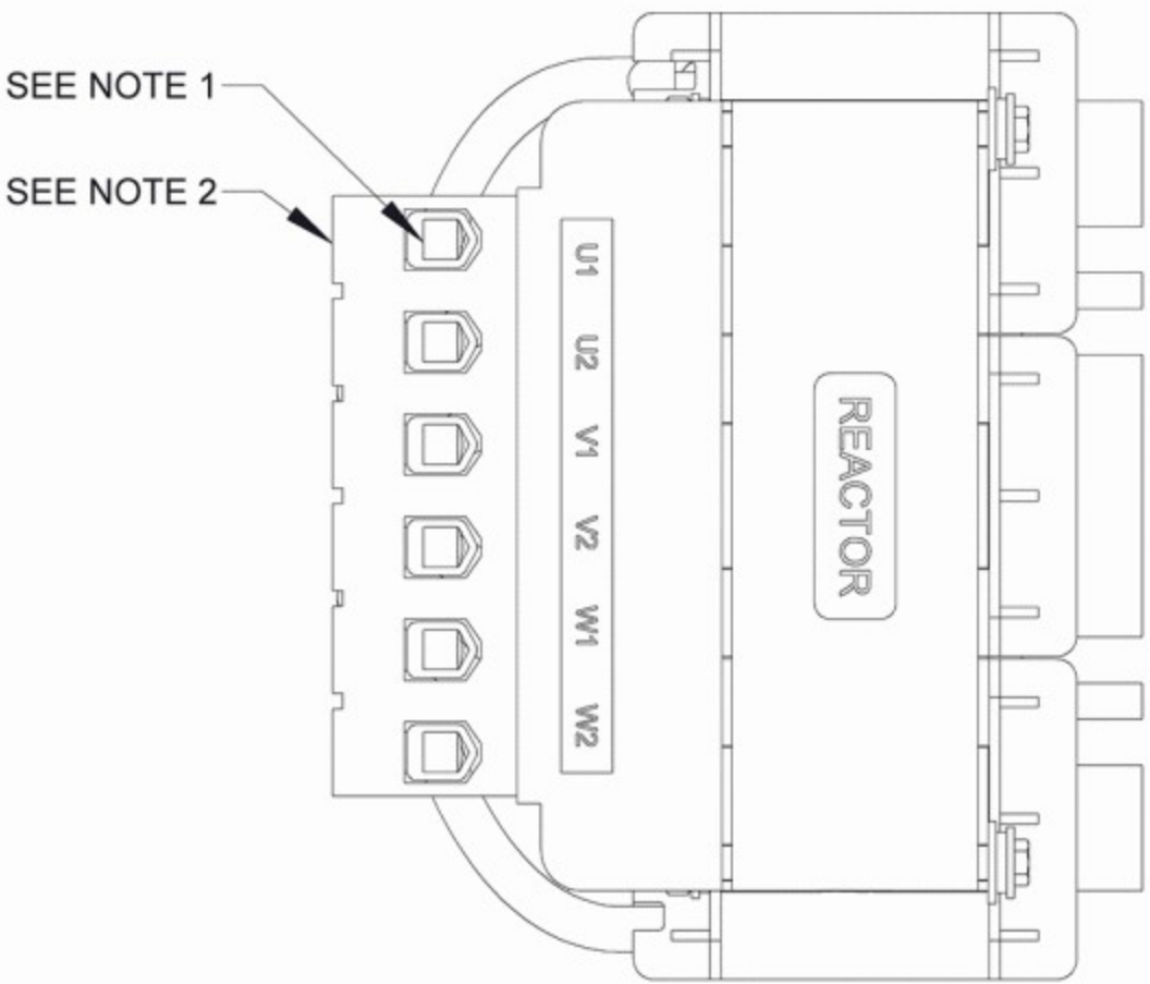
CUSTOMER CONNECTION DETAIL VIEW
