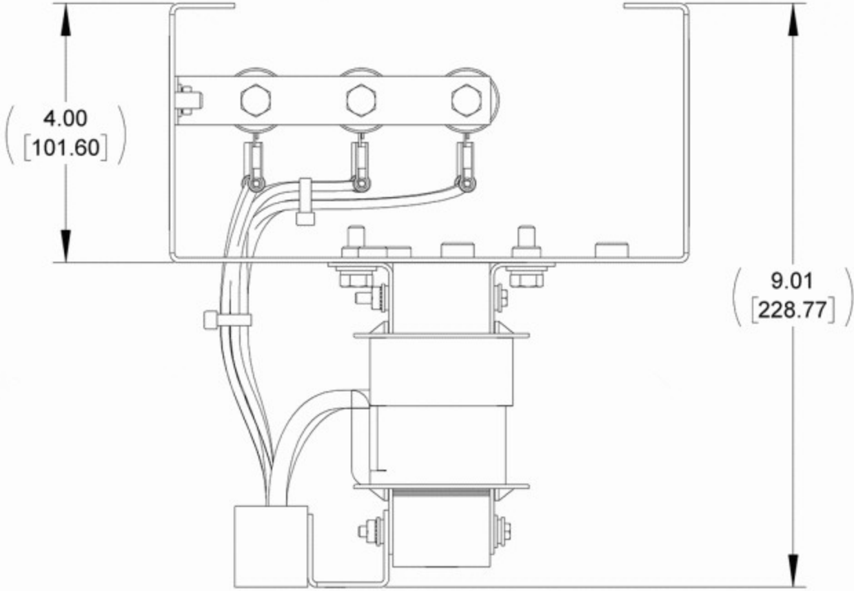
TOP VIEW
