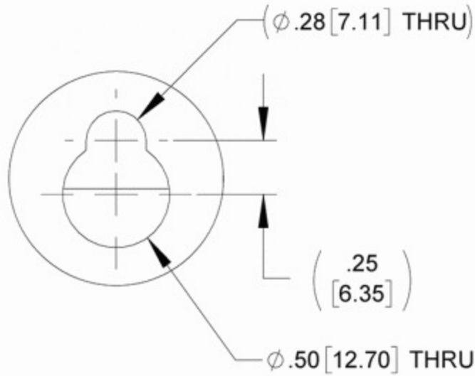
DETAIL A (2 PLACES)
