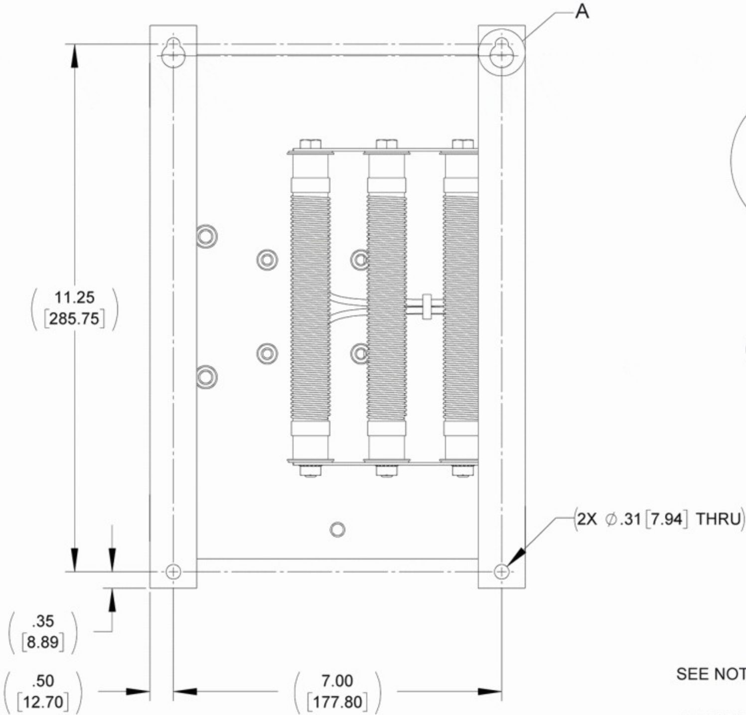
BACK VIEW
