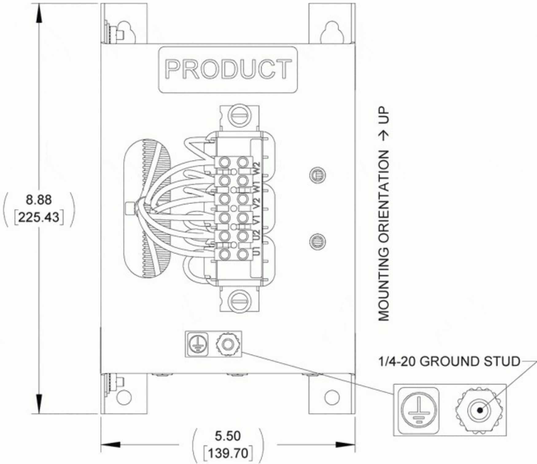
FRONT VIEW
