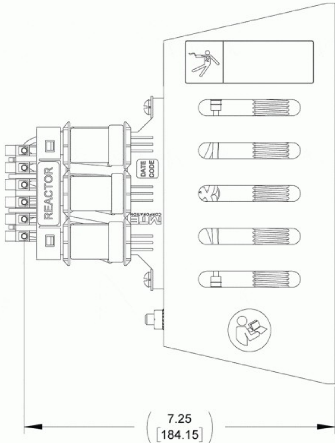
SIDE VIEW
