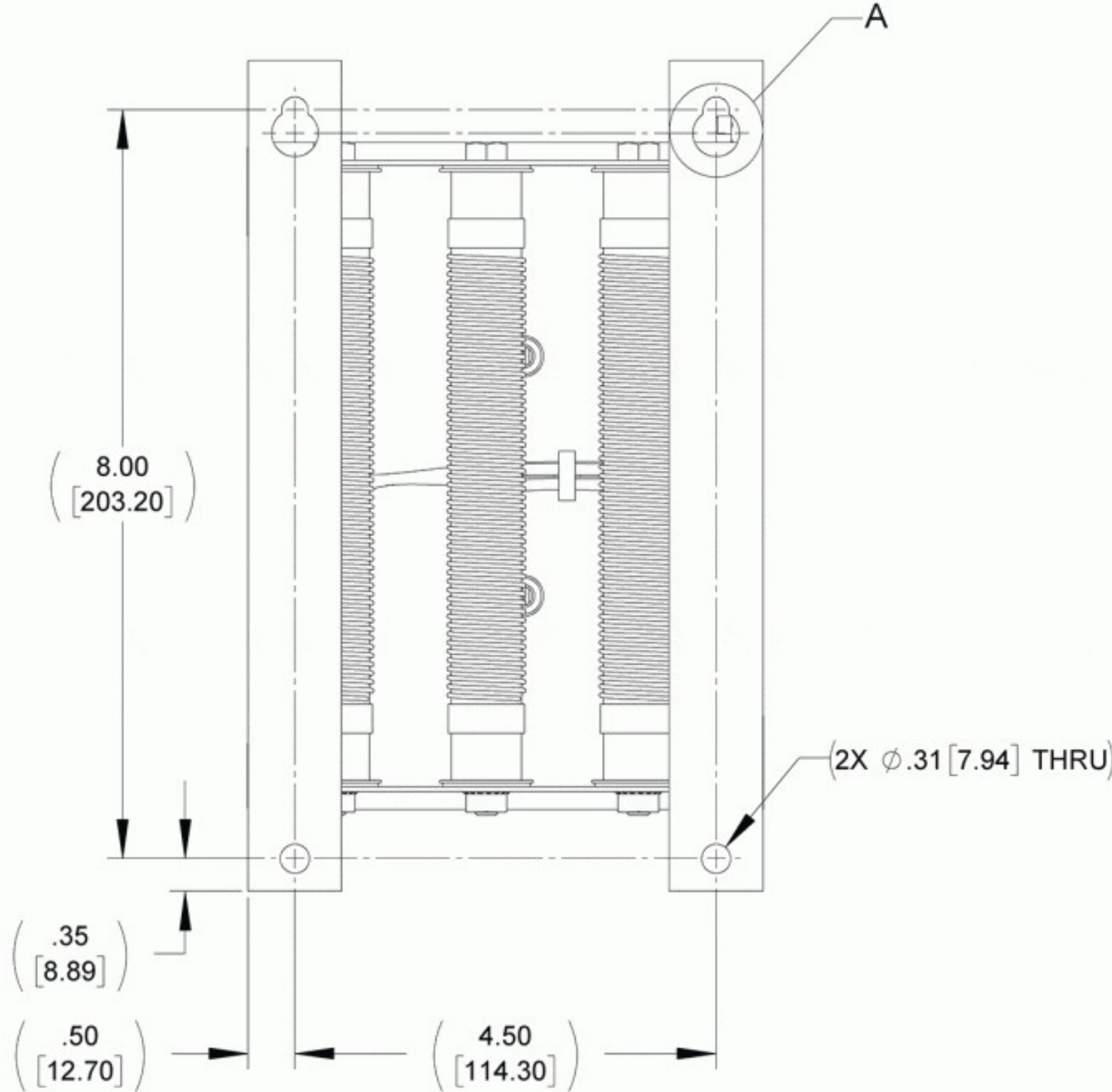
BACK VIEW
