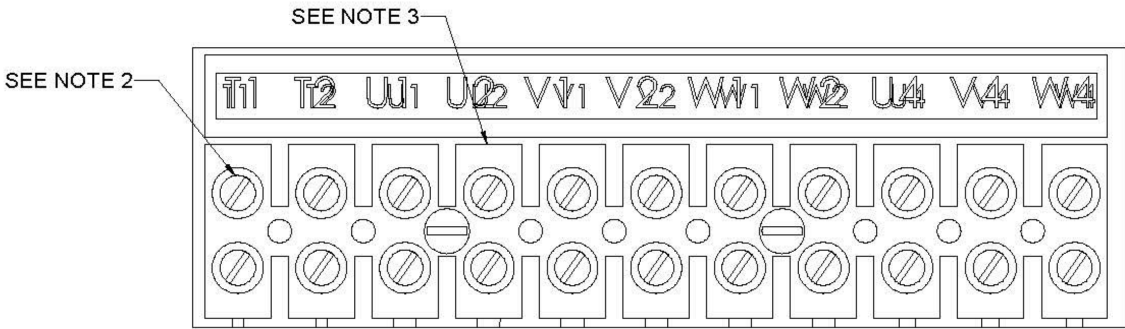
DETAIL A CUSTOMER CONNECTION DETAIL VIEW
