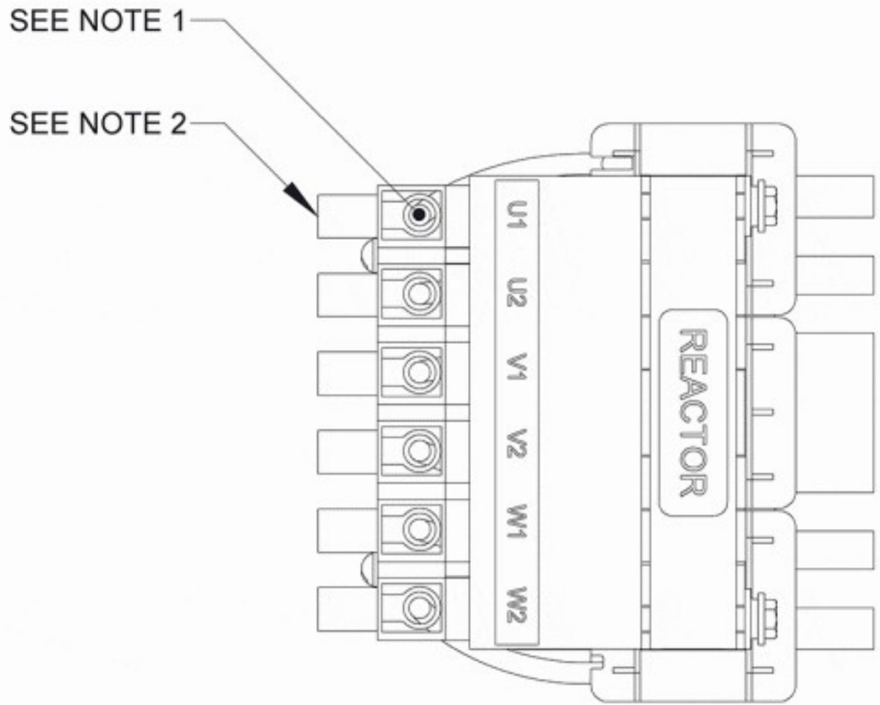
CUSTOMER CONNECTION DETAIL VIEW
